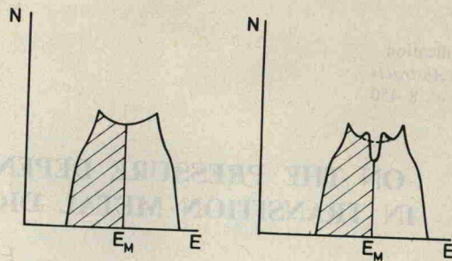
FIG. 2. — Density of states of the d band (schematic): a) normal undistorted phase; b) superlattice phase.
