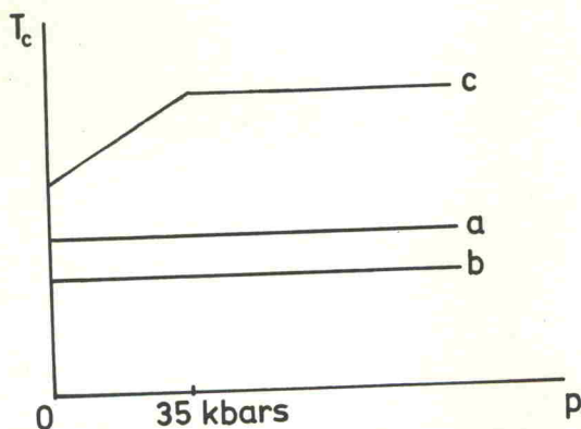
FIG. 1. — Pressure dependence of the critical temperature T_c in transition metal dichalcogenide layer compounds (schematic) : a) 2H\text{ Nb S}_2 ; b) 3R\text{ Nb S}_2 ; c) 2H\text{ Nb Se}_2 .
